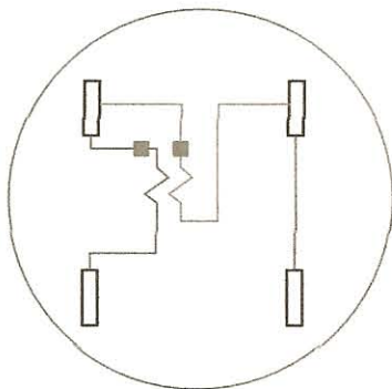
2-Wire FORM 1S
