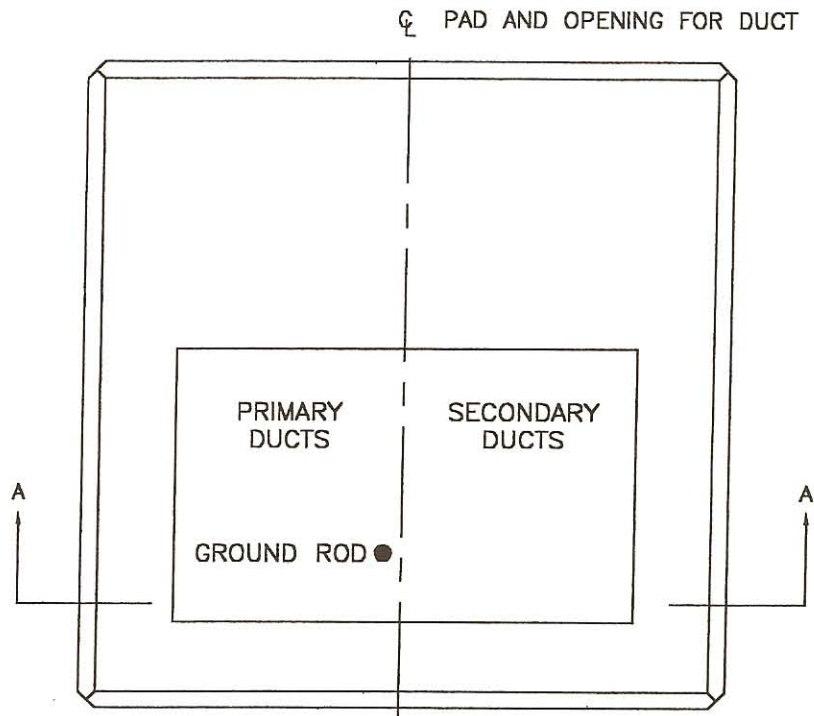
PEDESTAL PLAN
