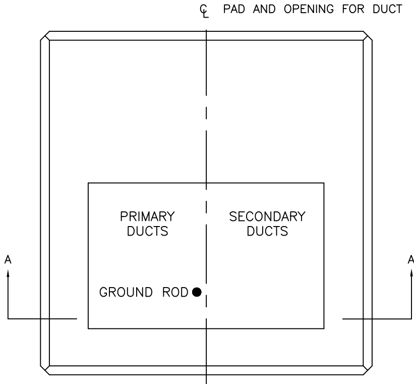
PEDESTAL PLAN
